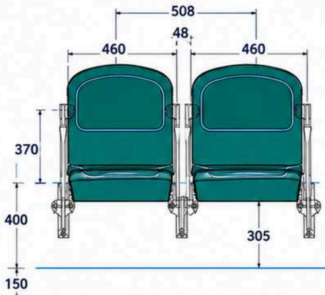
DIMENSION SPECIFICATIONS (All dimensions in millimetres)
