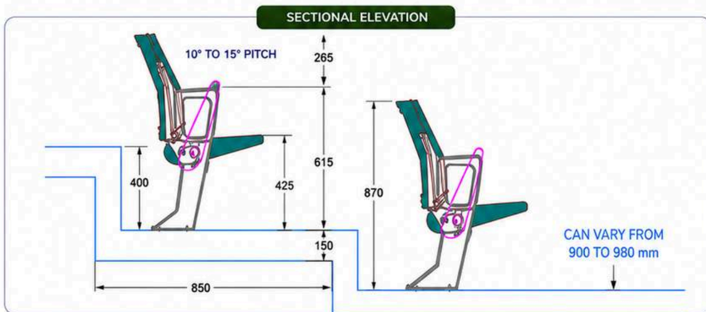
DIMENSION SPECIFICATIONS (All dimensions in millimetres)
