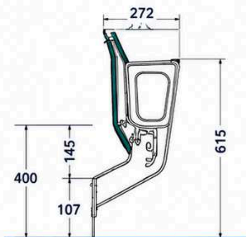
ALUMINIUM CASTING STAND
