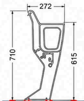
ALUMINIUM CASTING STAND
